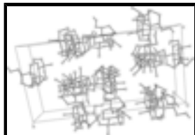
Fig. 3. A perspective view along the a-axis of the crystal packing of the title compound. The O-H...O hydrogen bonds are shown as dashed lines (see Table 1 for details).
