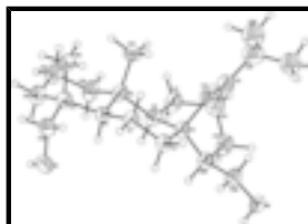
Fig. 1. A view of the molecular structure of one of the four independent molecules of the title compound. The displacement ellipsoids are drawn at the 30% probability level.
