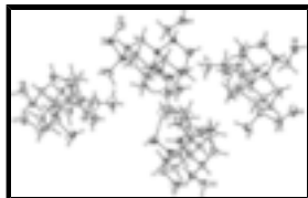
Fig. 2. A view of the four independent molecules of the title compound. The displacement ellipsoids are drawn at the 30% probability level.
